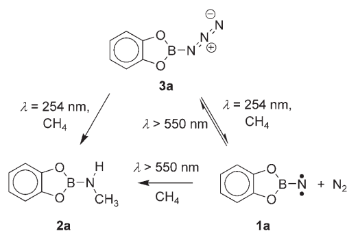
Scheme 1. Photochemistry of azidoborane 3a in an argon matrix doped with 1–2% methane.
