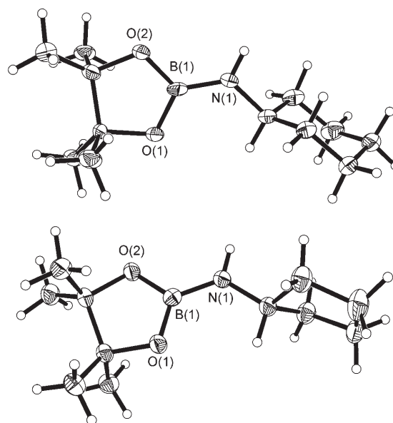
Figure 2. Single-crystal structure of 2b-cy6 (top) and 2b-cy5 (bottom) determined at 108 K and 113 K, respectively. [29] BN bond lengths: 1.386(4) Å ( 2b-cy6 ) and 1.393(2) Å ( 2b-cy5 ).
