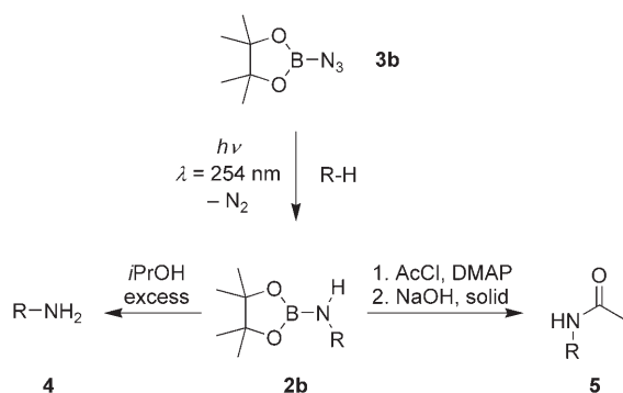
Scheme 3. Derivatization of aminoboranes 2b . DMAP = N,N' -dimethylaminopyridine, Ac = acetyl.
