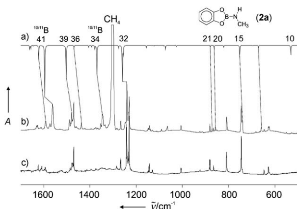
Figure 1. IR spectra obtained from the photolysis of azide 3a in solid argon at 10 K. a) IR spectrum computed for the C–H insertion product 2a at the B3LYP/6-311+G** level of theory. The numbers of the assigned vibrational modes (see Table S1 in the Supporting Information) are given on top. b) IR spectrum obtained after three photolysis cycles (254 nm followed by 550 nm) of 3a in the presence of CH 4 (2% in Ar). c) IR spectrum of borylnitrene 1a obtained in Ar in the absence of methane.
